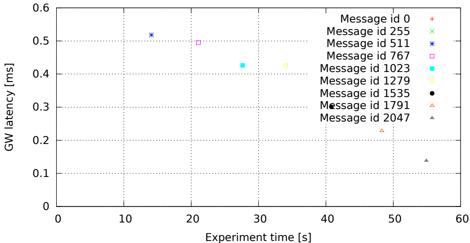
2048 GW rules (one per id, mask 0x7FF), no modifications (GW kernel 3.0.4-rt14-00008-gb2052fd, Traffic 50, Load cpu)
