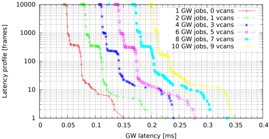
Chained GWs on multiple VCAN interfaces (GW kernel 3.0.4-00007-g1c8c373, Traffic onetatime, Load none)
