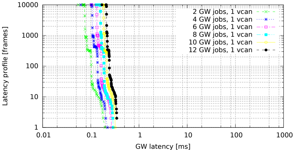
Chained GWs on a single VCAN interface (GW kernel 3.0.4-00007-g1c8c373, Traffic onetatime, Load none)
