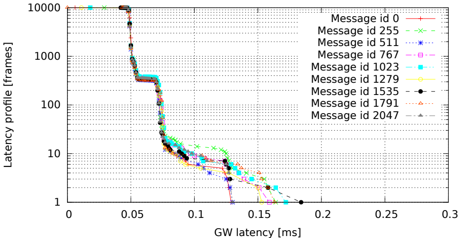
2048 GW rules (one per id, mask C00007FF), no modifications (GW kernel 3.0.4-00007-g1c8c373, Traffic oneatatime, Load none)
