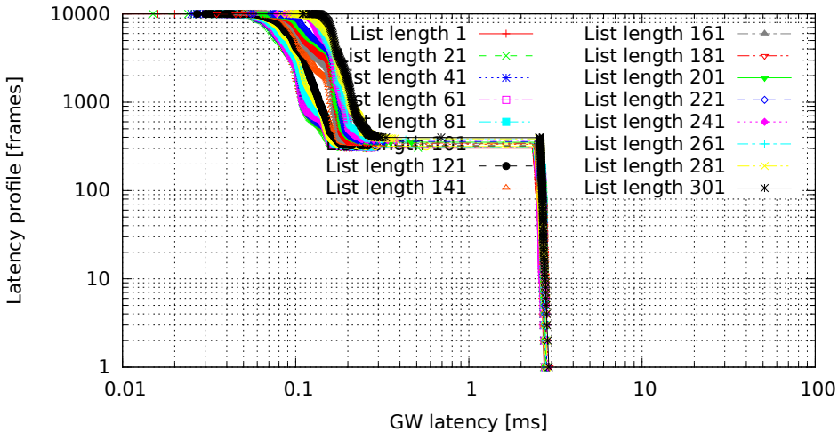
Different lengths of filter list, only the last one matches (GW kernel 3.0.4-00007-g1c8c373, Traffic oneatatime, Load eth)
