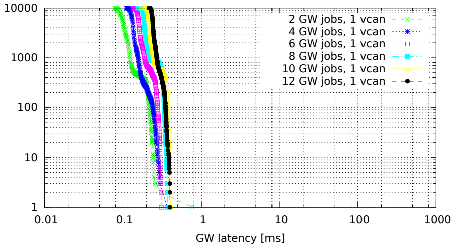
Chained GWs on a single VCAN interface (GW kernel 3.0.4-00007-g1c8c373, Traffic oneatatime, Load cpu)
