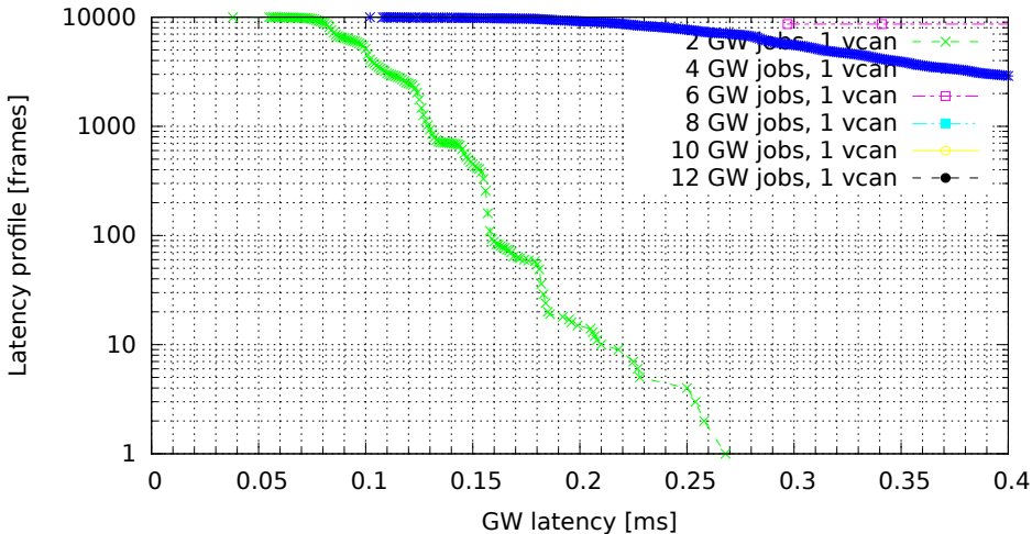
Chained GWs on a single VCAN interface (GW kernel 3.0.4-00007-g1c8c373, Traffic flood, Load none)
