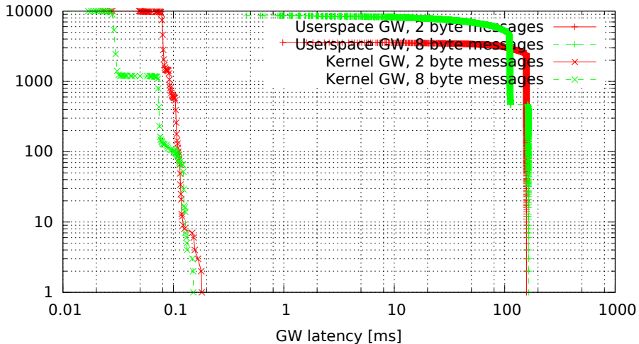
Kernel vs. userspace GW, no modifications (GW kernel 3.0.4-00007-g1c8c373, Traffic flood, Load none)
