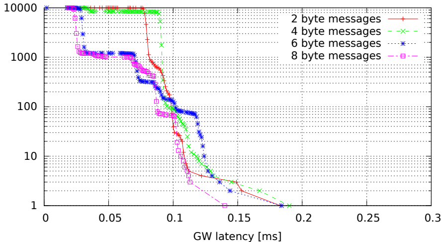
Single GW rule for all messages, no modifications (GW kernel 3.0.4-00007-g1c8c373, Traffic flood, Load none)
