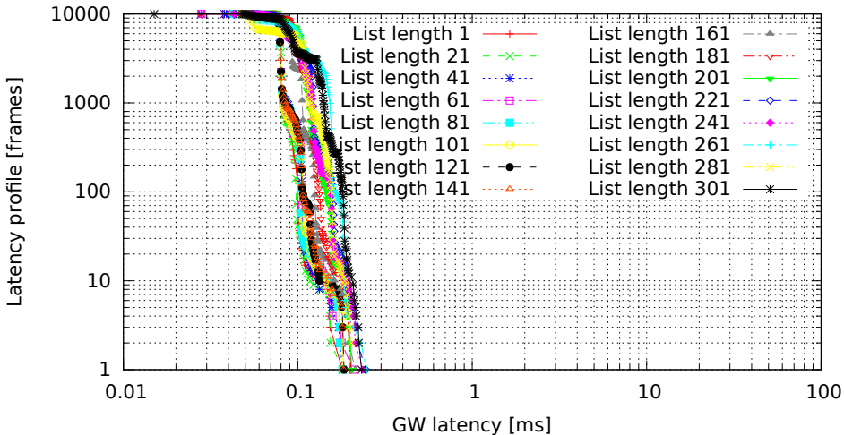
Different lengths of filter list, only the last one matches (GW kernel 3.0.4-00007-g1c8c373, Traffic flood, Load none)
