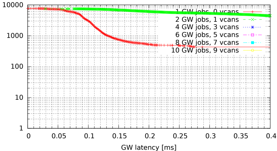
Chained GWs on multiple VCAN interfaces (GW kernel 3.0.4-00007-g1c8c373, Traffic flood, Load eth)
