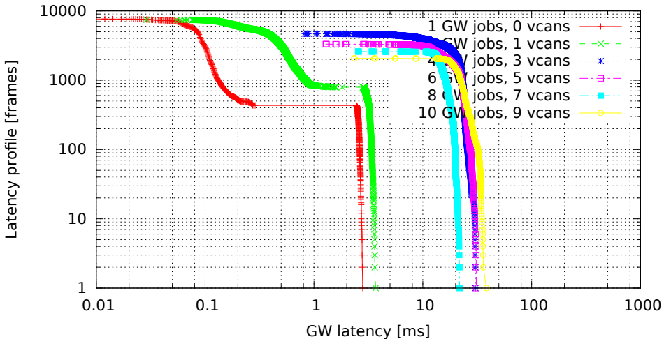
Chained GWs on multiple VCAN interfaces (GW kernel 3.0.4-00007-g1c8c373, Traffic flood, Load eth)
