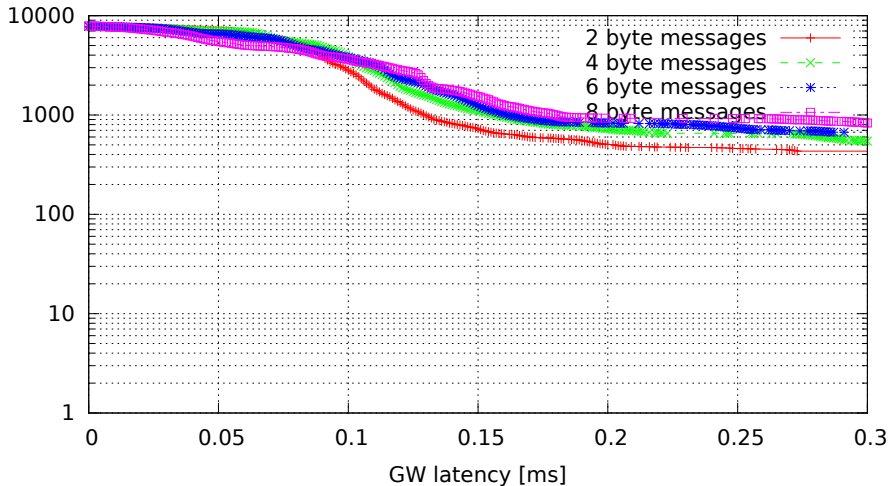
Single GW rule for all messages, no modifications (GW kernel 3.0.4-00007-g1c8c373, Traffic flood, Load eth)
