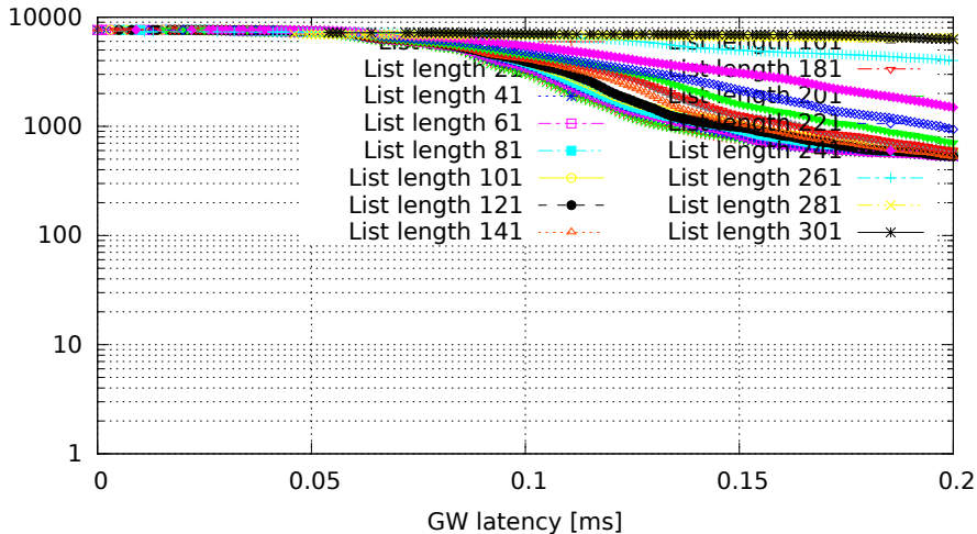
Different lengths of filter list, only the last one matches (GW kernel 3.0.4-00007-g1c8c373, Traffic flood, Load eth)
