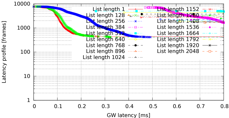
Different lengths of filter list, only the last one matches (GW kernel 3.0.4-00007-g1c8c373, Traffic flood, Load eth)
