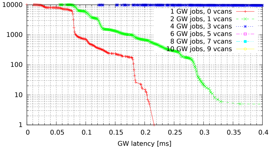
Chained GWs on multiple VCAN interfaces (GW kernel 3.0.4-00007-g1c8c373, Traffic flood, Load cpu)
