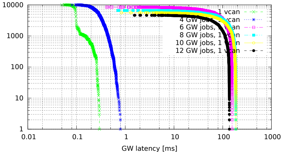
Chained GWs on a single VCAN interface (GW kernel 3.0.4-00007-g1c8c373, Traffic flood, Load cpu)
