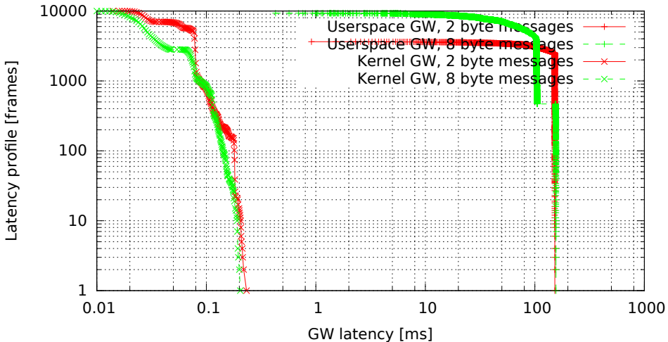
Kernel vs. userspace GW, no modifications (GW kernel 3.0.4-00007-g1c8c373, Traffic flood, Load cpu)
