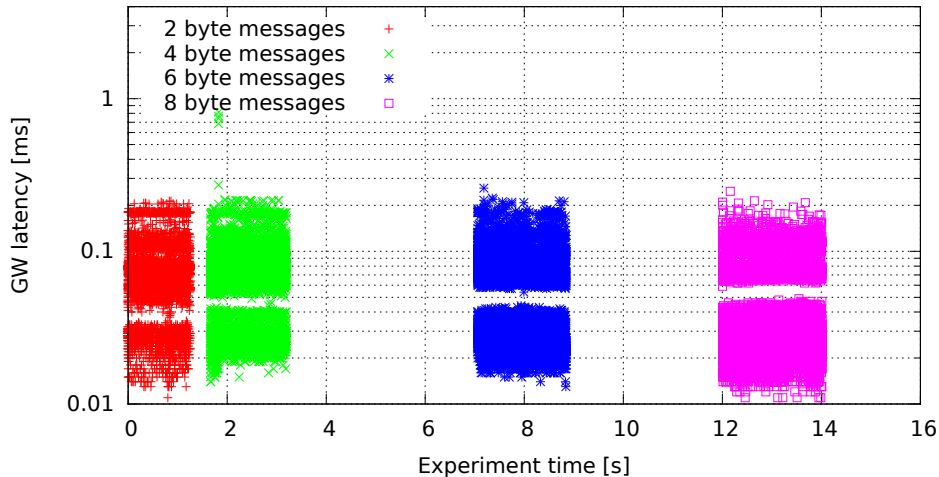
Single GW rule for all messages, no modifications, high (soft)irq task priority (GW kernel 3.0.4-00007-g1c8c373, Traffic flood, Load cpu)
