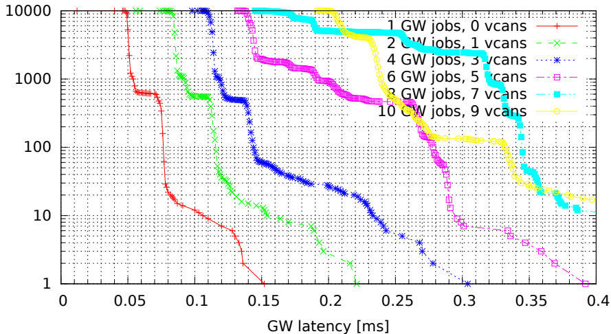
Chained GWs on multiple VCAN interfaces (GW kernel 3.0.4-00007-g1c8c373, Traffic 50, Load none)
