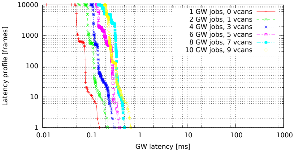
Chained GWs on multiple VCAN interfaces (GW kernel 3.0.4-00007-g1c8c373, Traffic 50, Load none)
