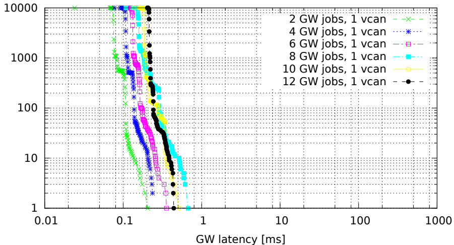
Chained GWs on a single VCAN interface (GW kernel 3.0.4-00007-g1c8c373, Traffic 50, Load none)
