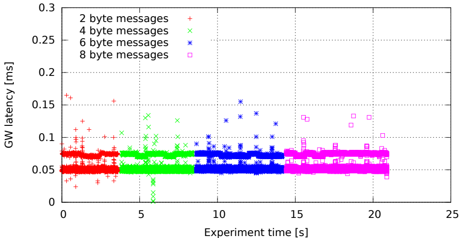
Single GW rule for all messages, no modifications, high (soft)irq task priority (GW kernel 3.0.4-00007-g1c8c373, Traffic 50, Load none)
