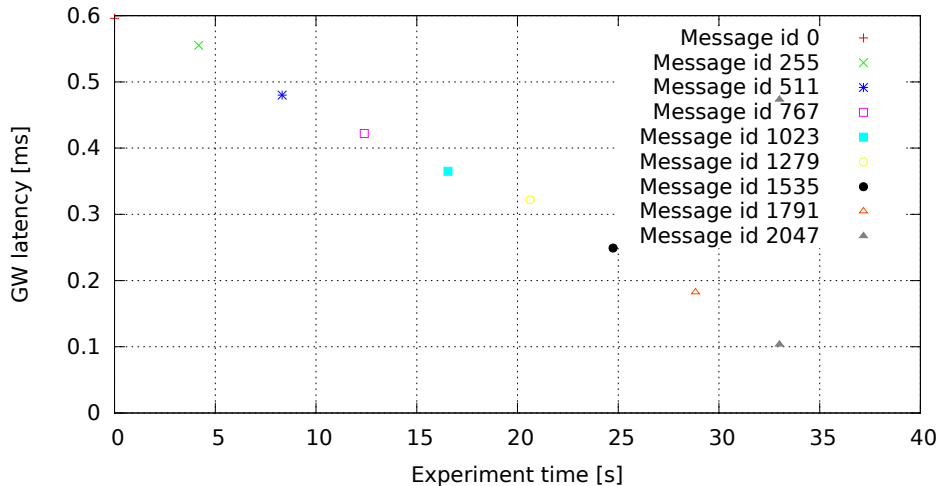
2048 GW rules (one per id, mask 0x7FF), no modifications (GW kernel 3.0.4-00007-g1c8c373, Traffic 50, Load none)
