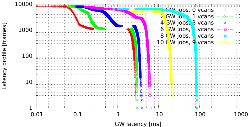
Chained GWs on multiple VCAN interfaces (GW kernel 3.0.4-00007-g1c8c373, Traffic 50, Load eth)
