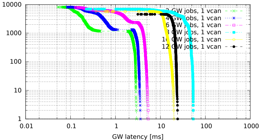
Chained GWs on a single VCAN interface (GW kernel 3.0.4-00007-g1c8c373, Traffic 50, Load eth)
