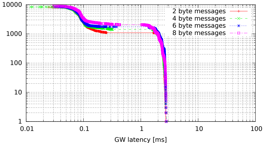
Single GW rule for all messages, no modifications (GW kernel 3.0.4-00007-g1c8c373, Traffic 50, Load eth)
