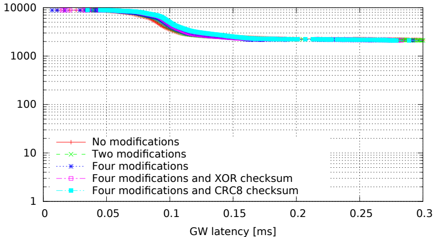
Single GW rule for all messages with modifications, 8 byte messages (GW kernel 3.0.4-00007-g1c8c373, Traffic 50, Load eth)
