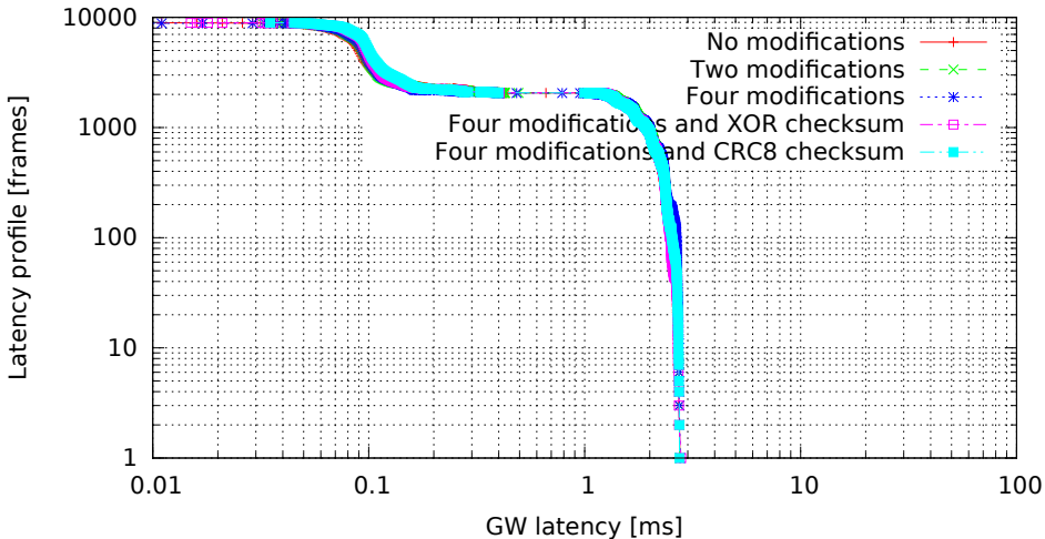
Single GW rule for all messages with modifications, 8 byte messages (GW kernel 3.0.4-00007-g1c8c373, Traffic 50, Load eth)
