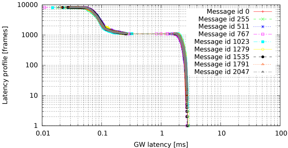
2048 GW rules (one per id, mask C0007FF), no modifications (GW kernel 3.0.4-00007-g1c8c373, Traffic 50, Load eth)
