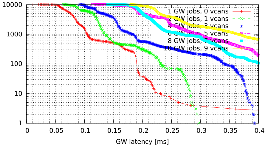
Chained GWs on multiple VCAN interfaces (GW kernel 3.0.4-00007-g1c8c373, Traffic 50, Load cpu)
