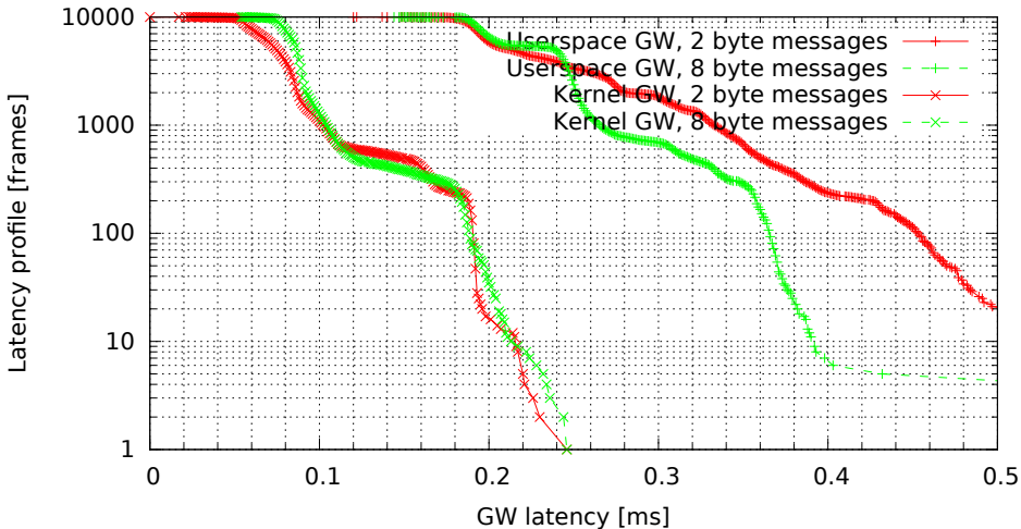
Kernel vs. userspace GW, no modifications (GW kernel 3.0.4-00007-g1c8c373, Traffic 50, Load cpu)
