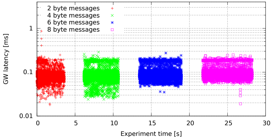
Single GW rule for all messages, no modifications, high (soft)irq task priority (GW kernel 3.0.4-00007-g1c8c373, Traffic 50, Load cpu)
