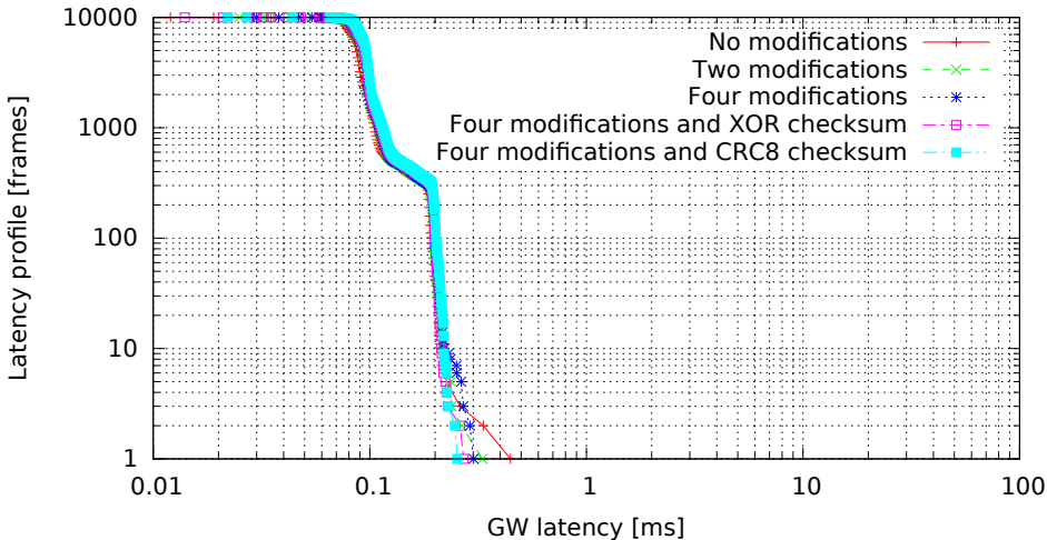
Single GW rule for all messages with modifications, 8 byte messages (GW kernel 3.0.4-00007-g1c8c373, Traffic 50, Load cpu)
