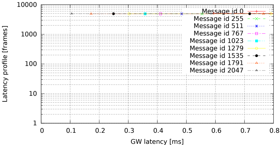
2048 GW rules (one per id, mask 0x7FF), no modifications (GW kernel 3.0.4-00007-g1c8c373, Traffic 50, Load cpu)
