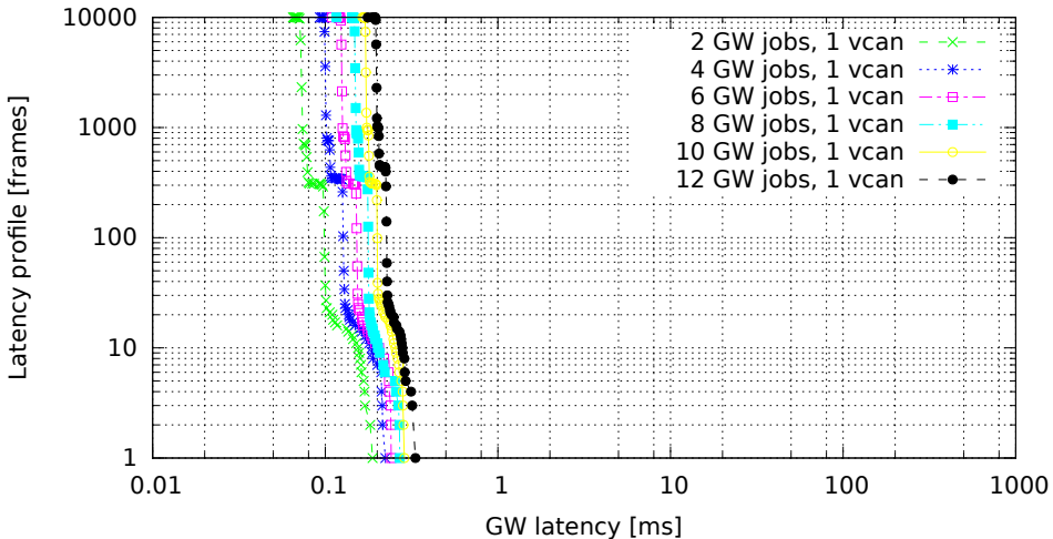
Chained GWs on a single VCAN interface (GW kernel 2.6.36.2-00015-g4f1bc4e, Traffic oneatatime, Load none)
