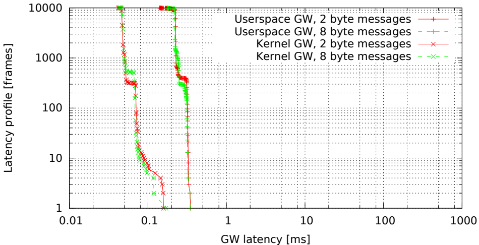
Kernel vs. userspace GW, no modifications (GW kernel 2.6.36.2-00015-g4f1bc4e, Traffic oneatatime, Load none)
