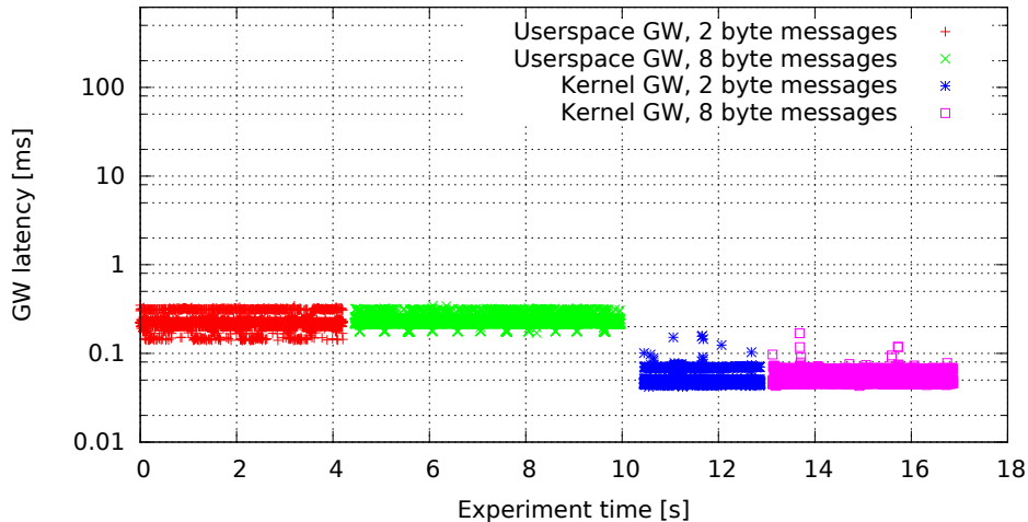
Single GW rule for all messages, no modifications (GW kernel 2.6.36.2-00015-g4f1bc4e, Traffic oneatatime, Load none)
