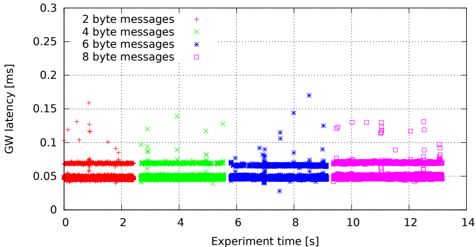
Single GW rule for all messages, no modifications, high (soft)irq task priority (GW kernel 2.6.36.2-00015-g4f1bc4e, Traffic oneatatime, Load none)
