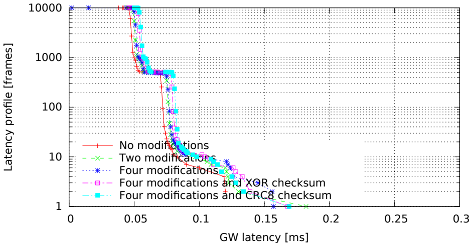
Single GW rule for all messages with modifications, 8 byte messages (GW kernel 2.6.36.2-00015-g4f1bc4e, Traffic oneatatime, Load none)
