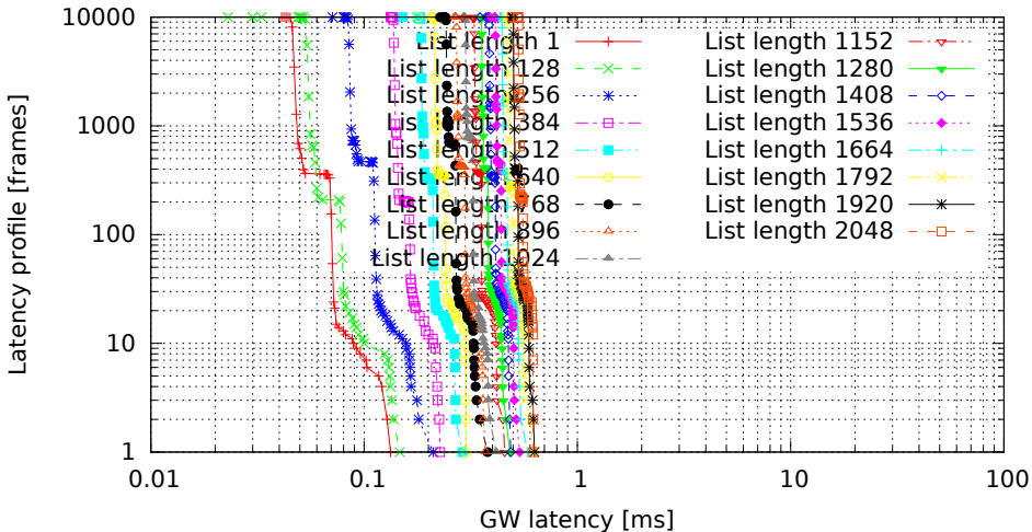
Different lengths of filter list, only the last one matches (GW kernel 2.6.36.2-00015-g4f1bc4e, Traffic oneatatime, Load none)
