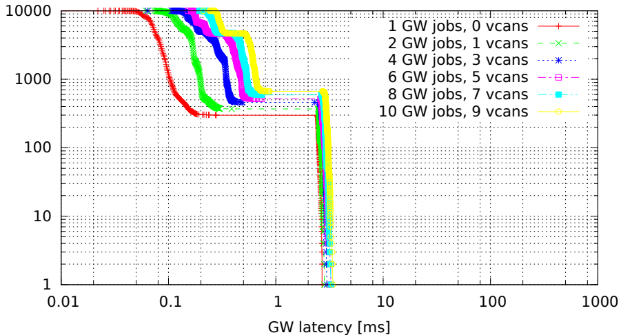
Chained GWs on multiple VCAN interfaces (GW kernel 2.6.36.2-00015-g4f1bc4e, Traffic oneatatime, Load eth)
