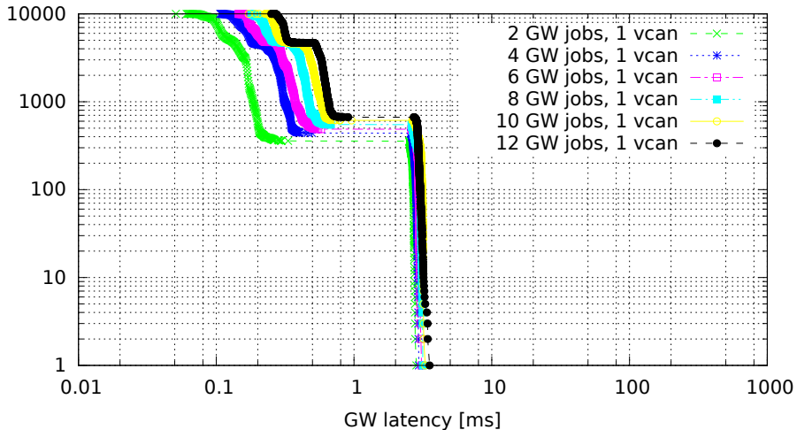
Chained GWs on a single VCAN interface (GW kernel 2.6.36.2-00015-g4f1bc4e, Traffic onetatime, Load eth)
