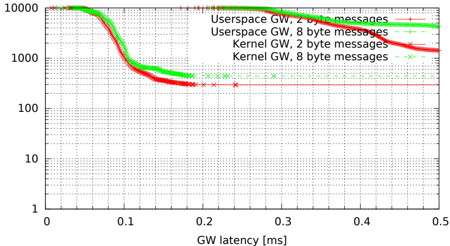
Kernel vs. userspace GW, no modifications (GW kernel 2.6.36.2-00015-g4f1bc4e, Traffic oneatatime, Load eth)
