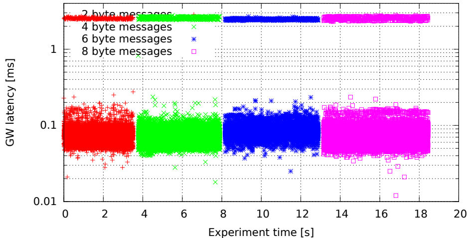
Single GW rule for all messages, no modifications (GW kernel 2.6.36.2-00015-g4f1bc4e, Traffic oneatatime, Load eth)
