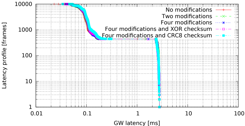
Single GW rule for all messages with modifications, 8 byte messages (GW kernel 2.6.36.2-00015-g4f1bc4e, Traffic onetotime, Load eth)
