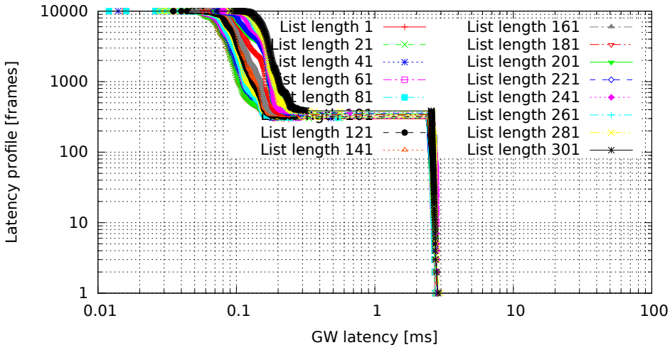
Different lengths of filter list, only the last one matches (GW kernel 2.6.36.2-00015-g4f1bc4e, Traffic oneatatime, Load eth)
