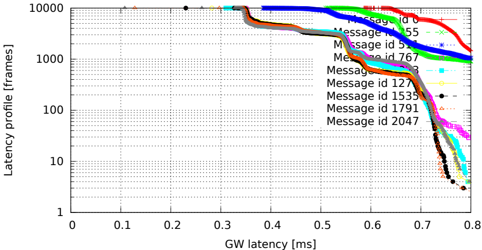
2048 GW rules (one per id, mask 0x7FF), no modifications (GW kernel 2.6.36.2-00015-g4f1bc4e, Traffic onetotime, Load eth)
