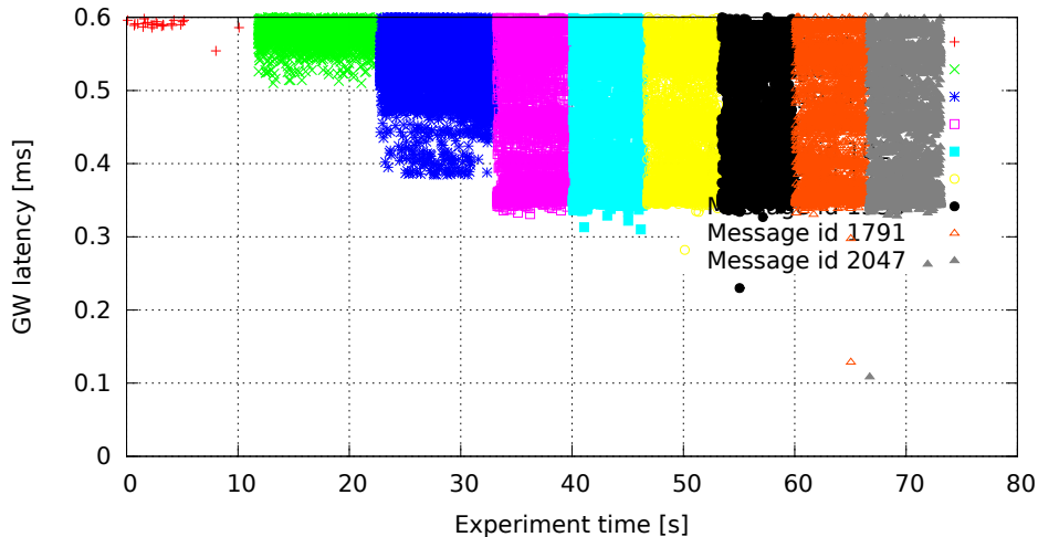
2048 GW rules (one per id, mask 0x7FF), no modifications (GW kernel 2.6.36.2-00015-g4f1bc4e, Traffic oneatatime, Load eth)
