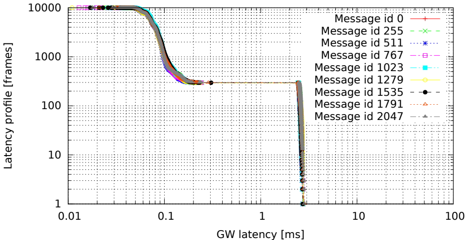
2048 GW rules (one per id, mask C00007FF), no modifications (GW kernel 2.6.36.2-00015-g4f1bc4e, Traffic onetatime, Load eth)
